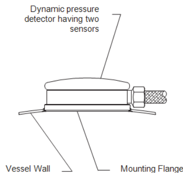
Dynamic Pressure Detector
